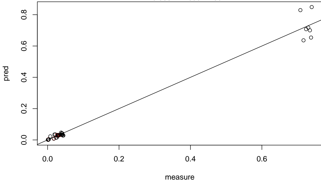
Model: 6-2-1
