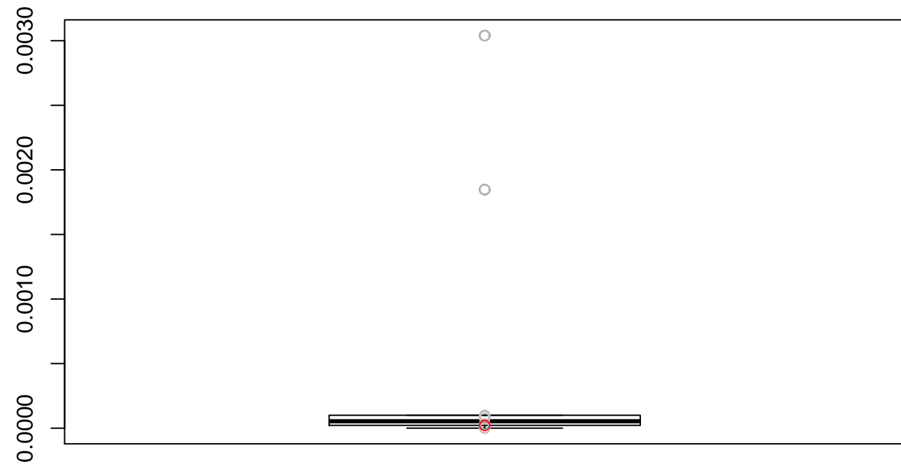
MSE: 0.000523565033030511
