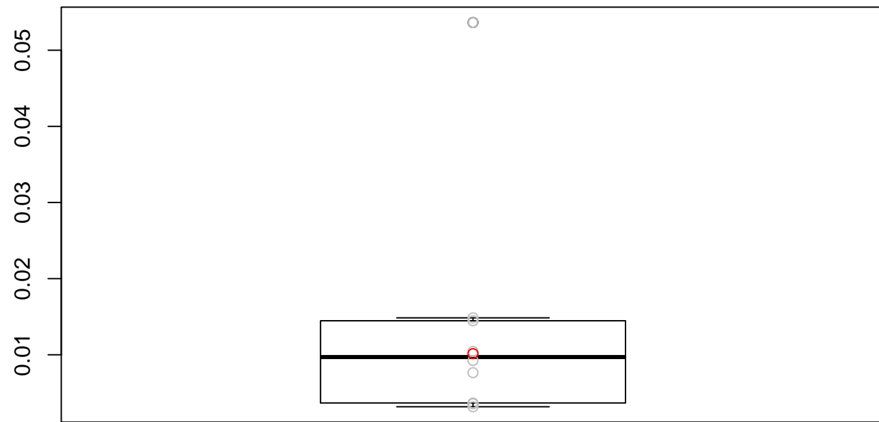
MSE: 0.0130875674938394
