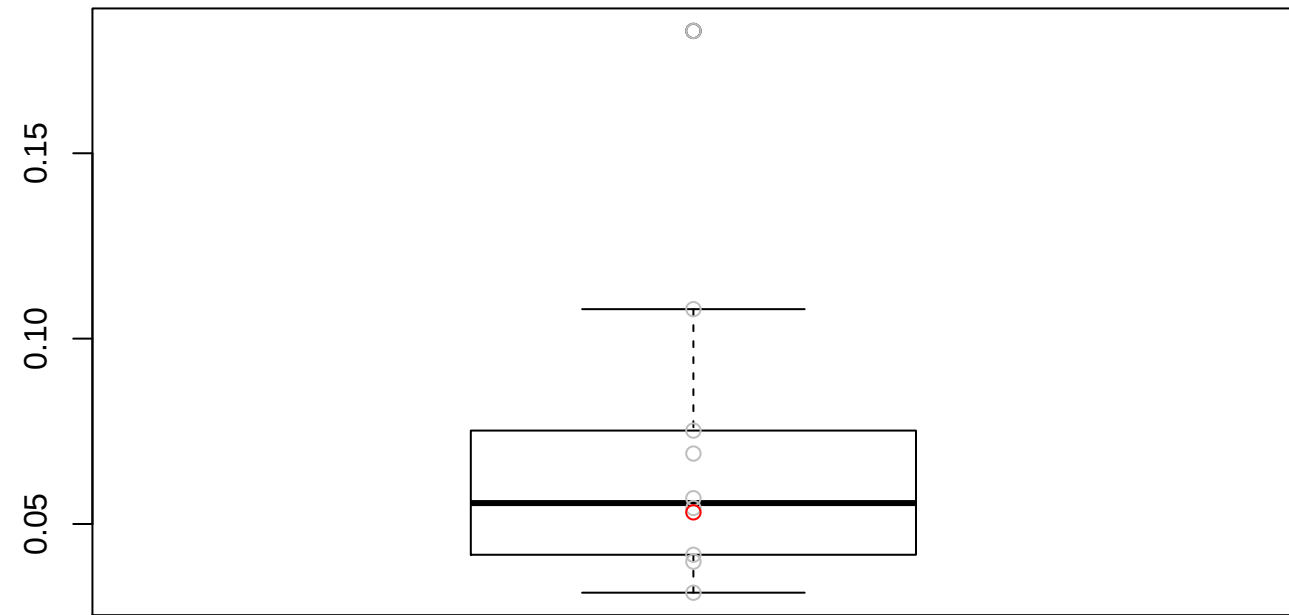
MSE: 0.0712609032251803
