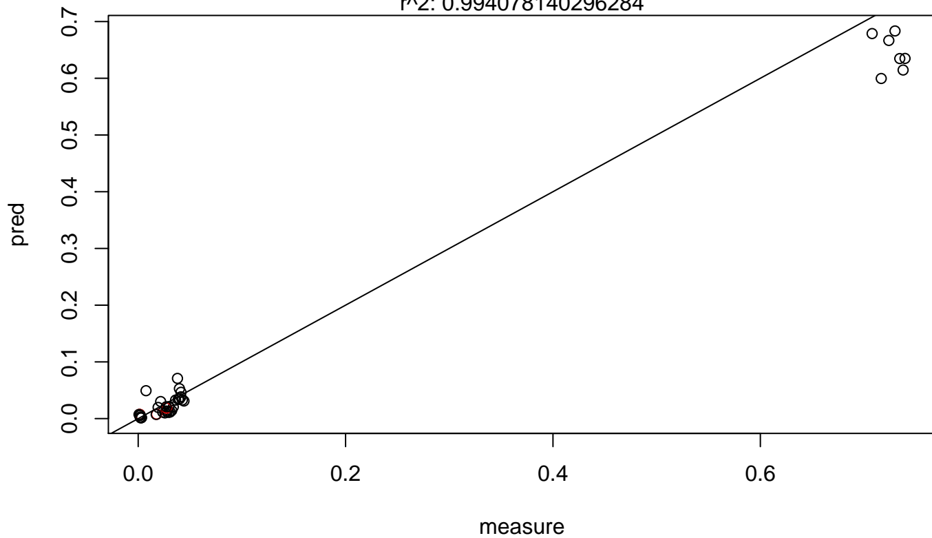
Model: 7-5-1
