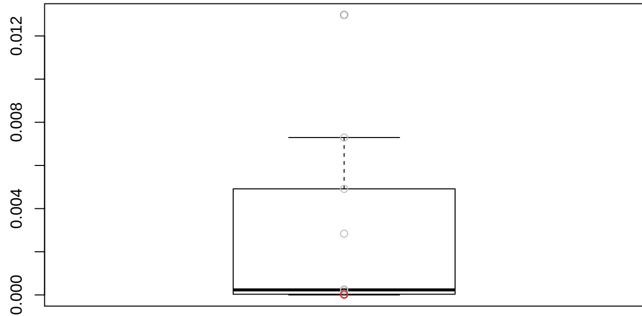
MSE: 0.00285973670054378
