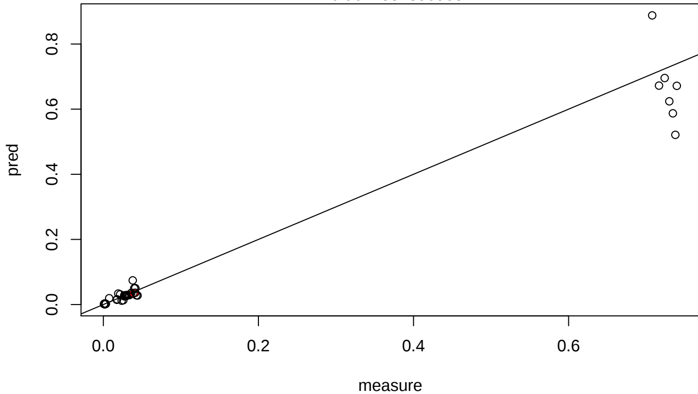
Model: 7-5-1
