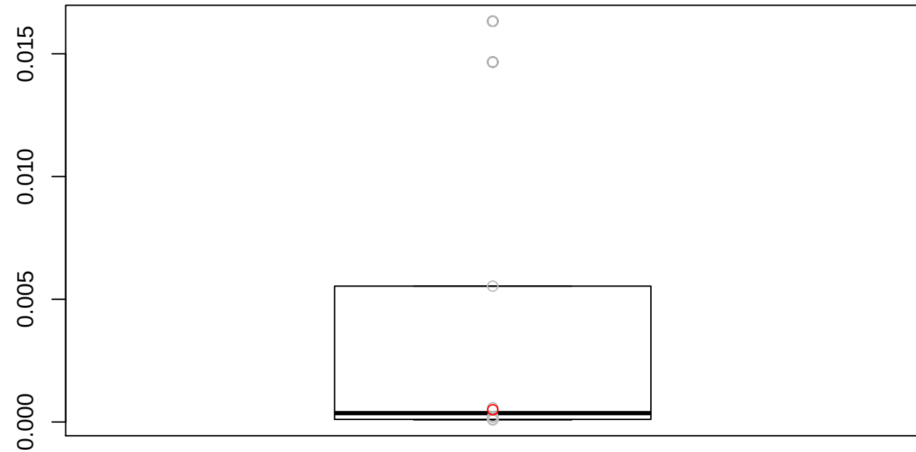
MSE: 0.00383078499172858
