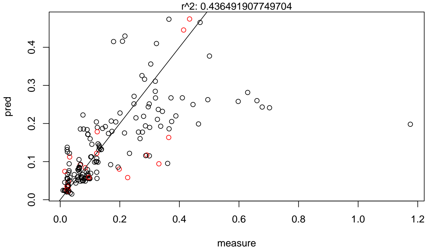
Model: 7-5-1
