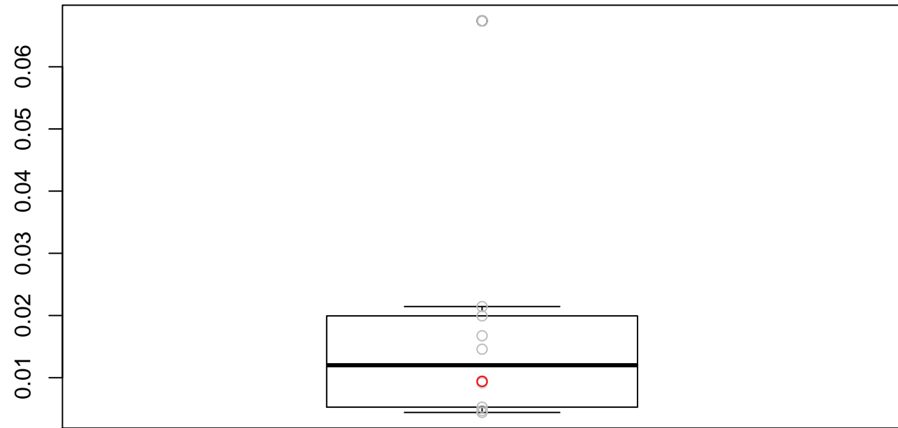
MSE: 0.0173066616858016
