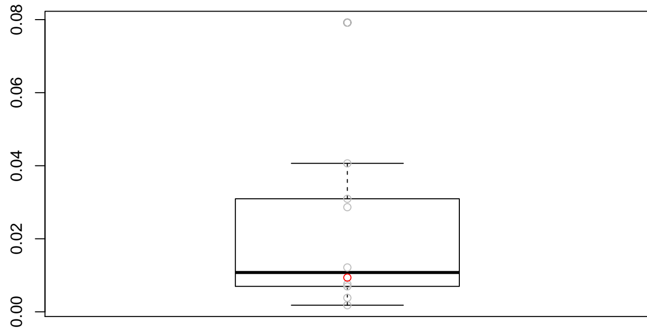
MSE: 0.0221163804159431
