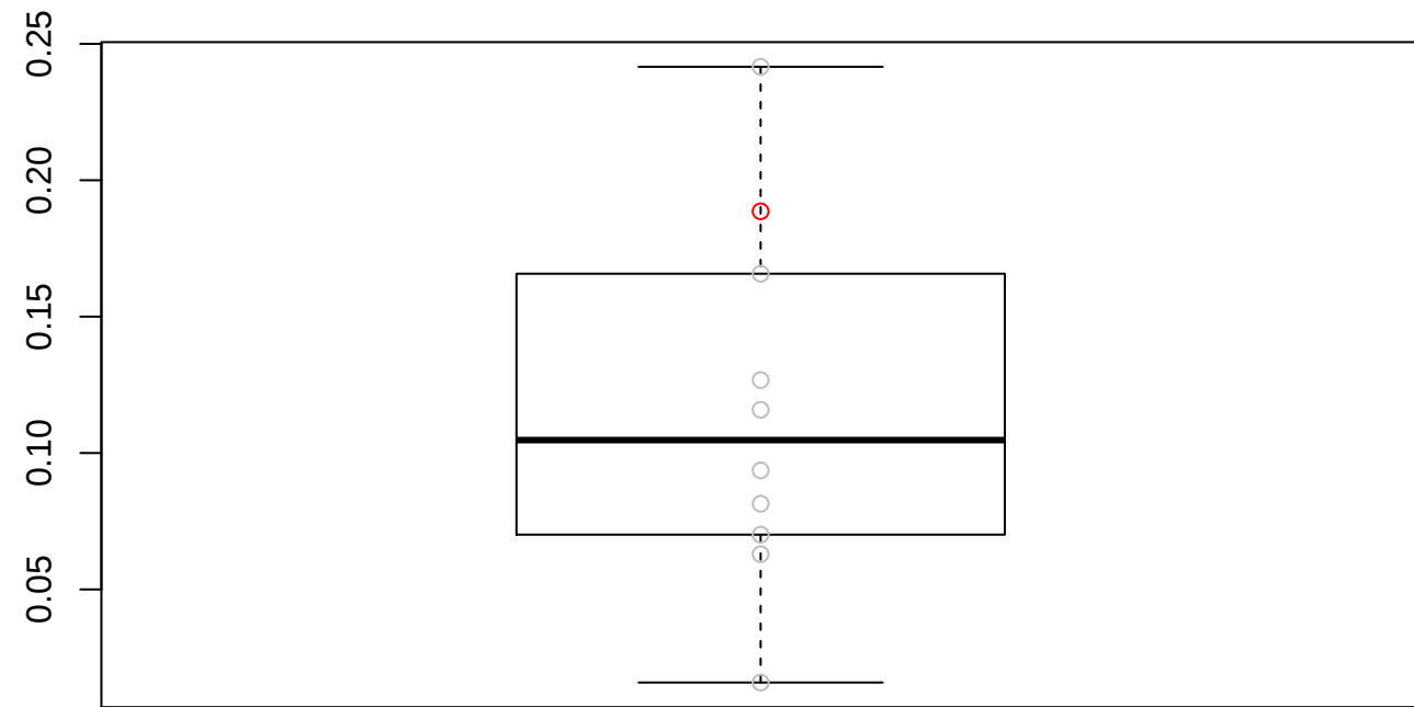
MSE: 0.116248837339892
