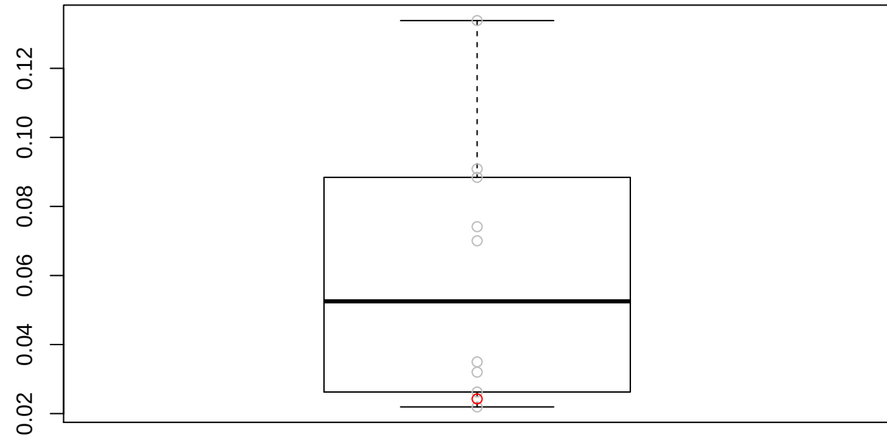
MSE: 0.059680522002217
