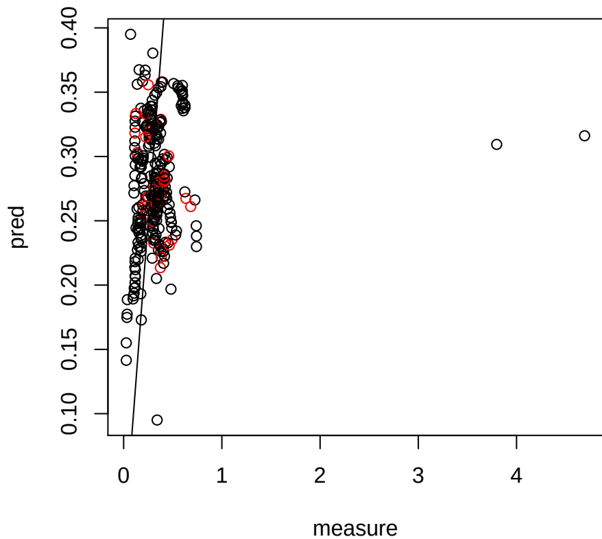
Model: 6-5-1
