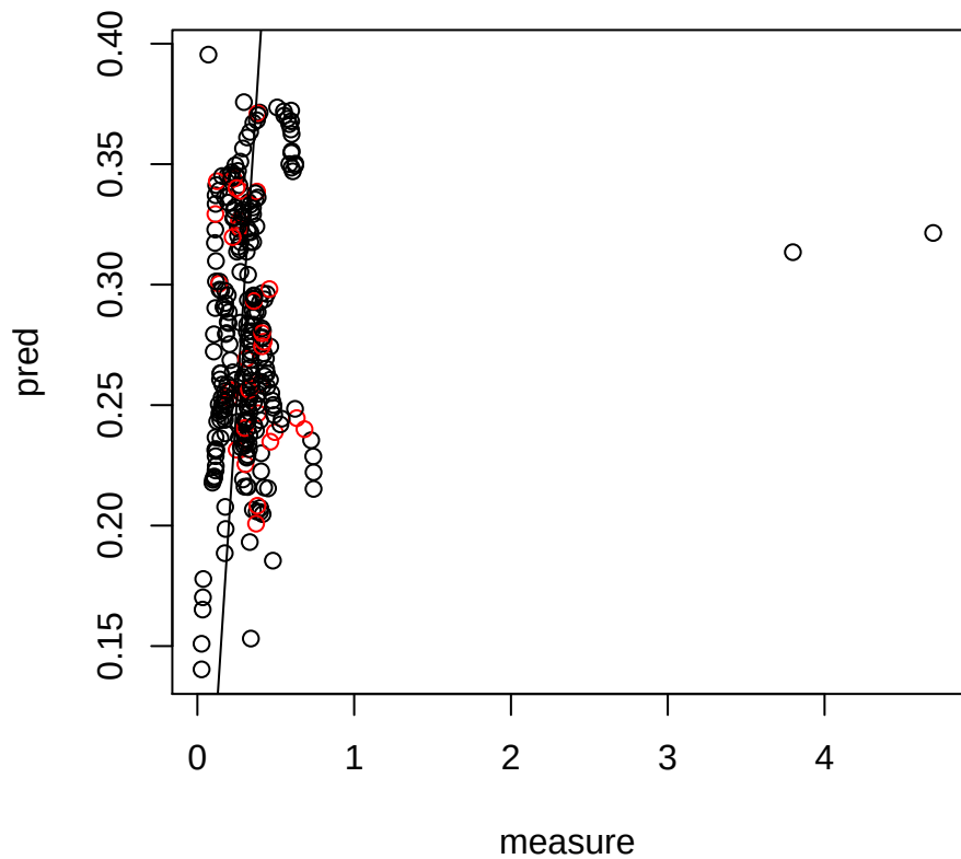
Model: 6-2-1
