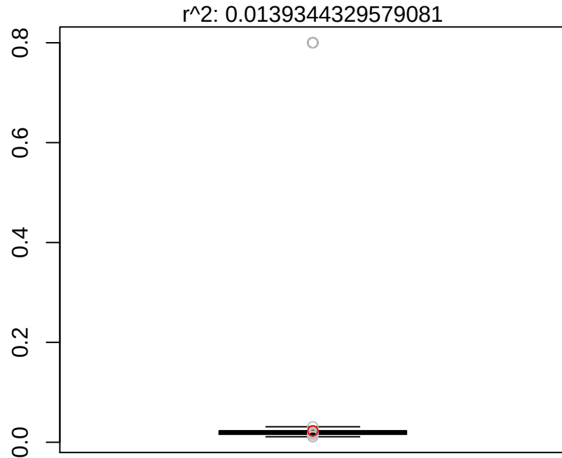
MSE: 0.0970334438099586
