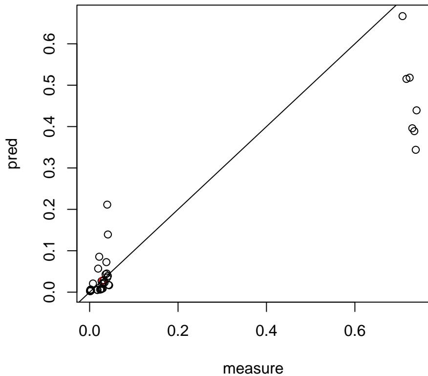
Model: 6-5-1
