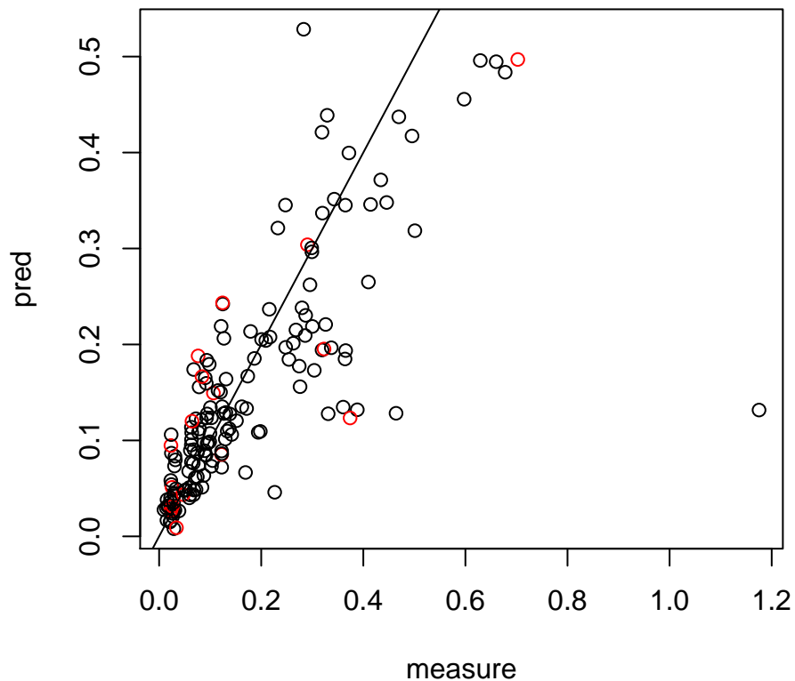
Model: 6-5-1
