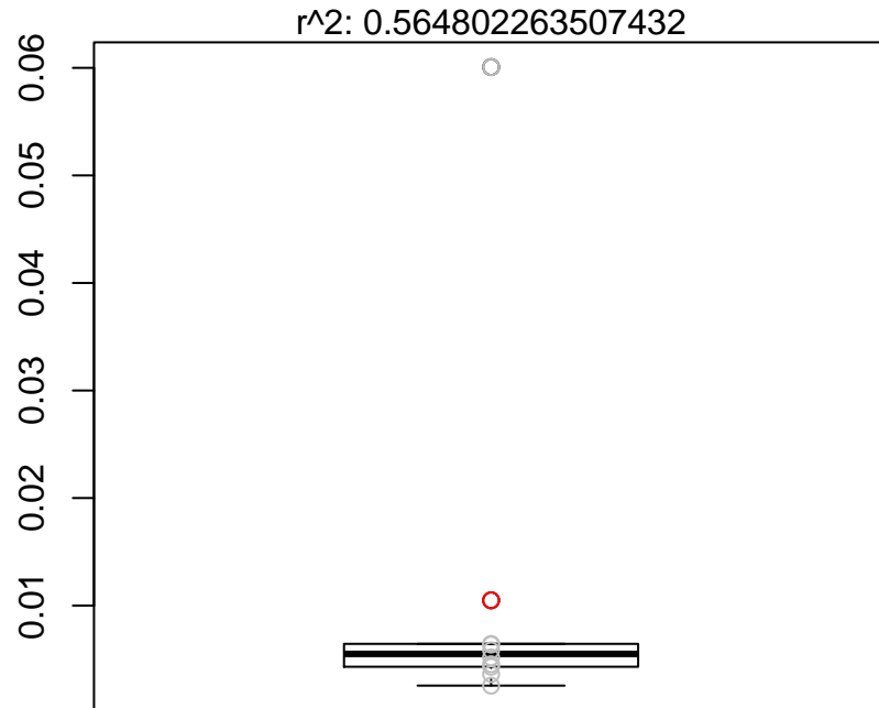
MSE: 0.010943895051086
