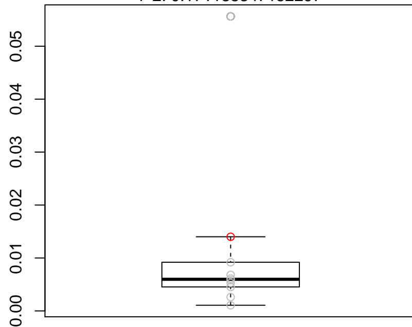
MSE: 0.0111075571754897
