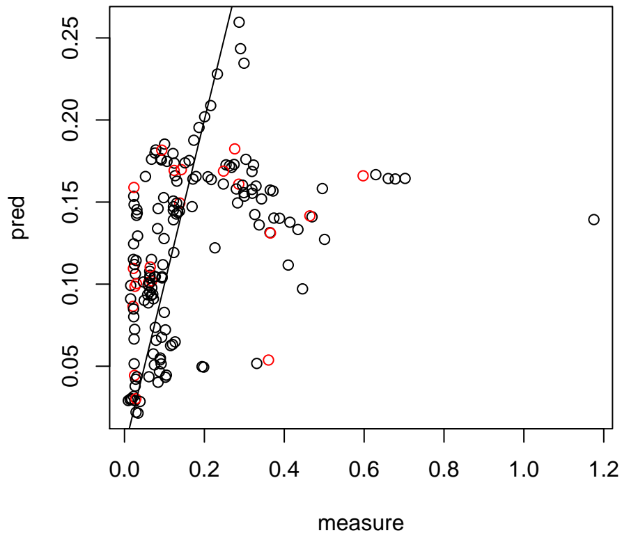
Model: 6-3-1
