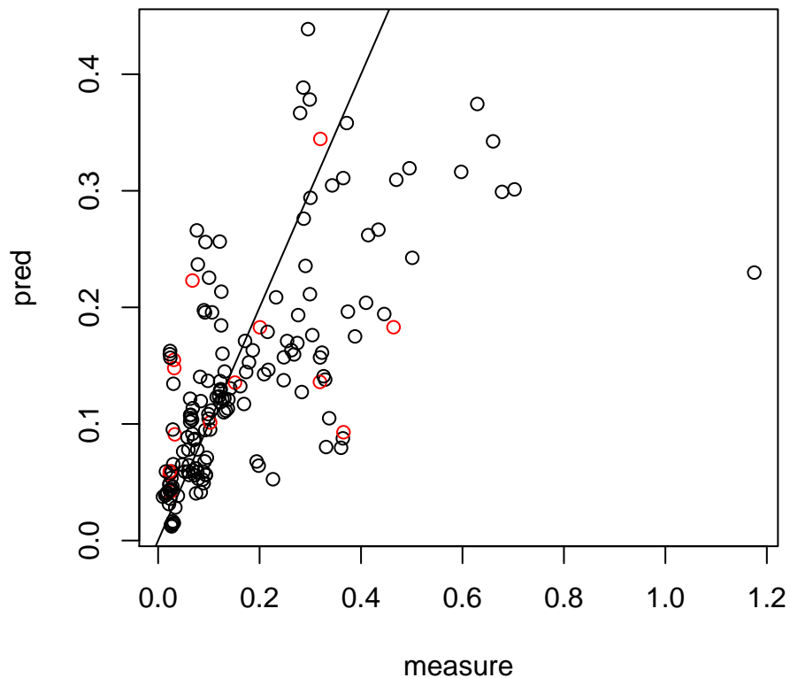
Model: 6-2-1
