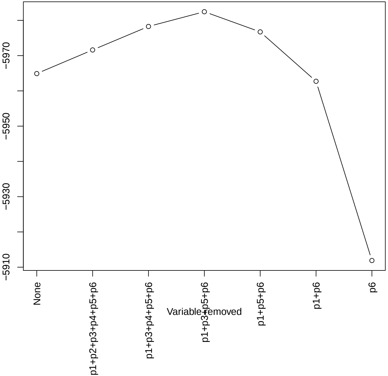
AIC v. variables (all)
