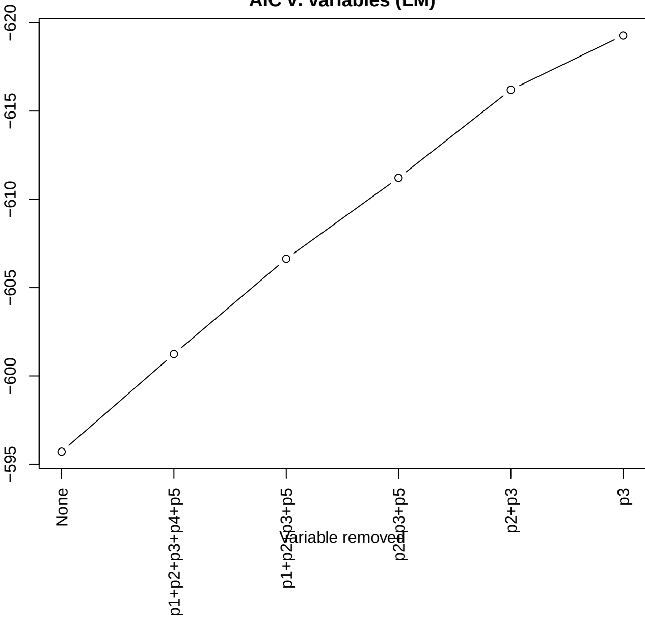
AIC v. variables (LM)
