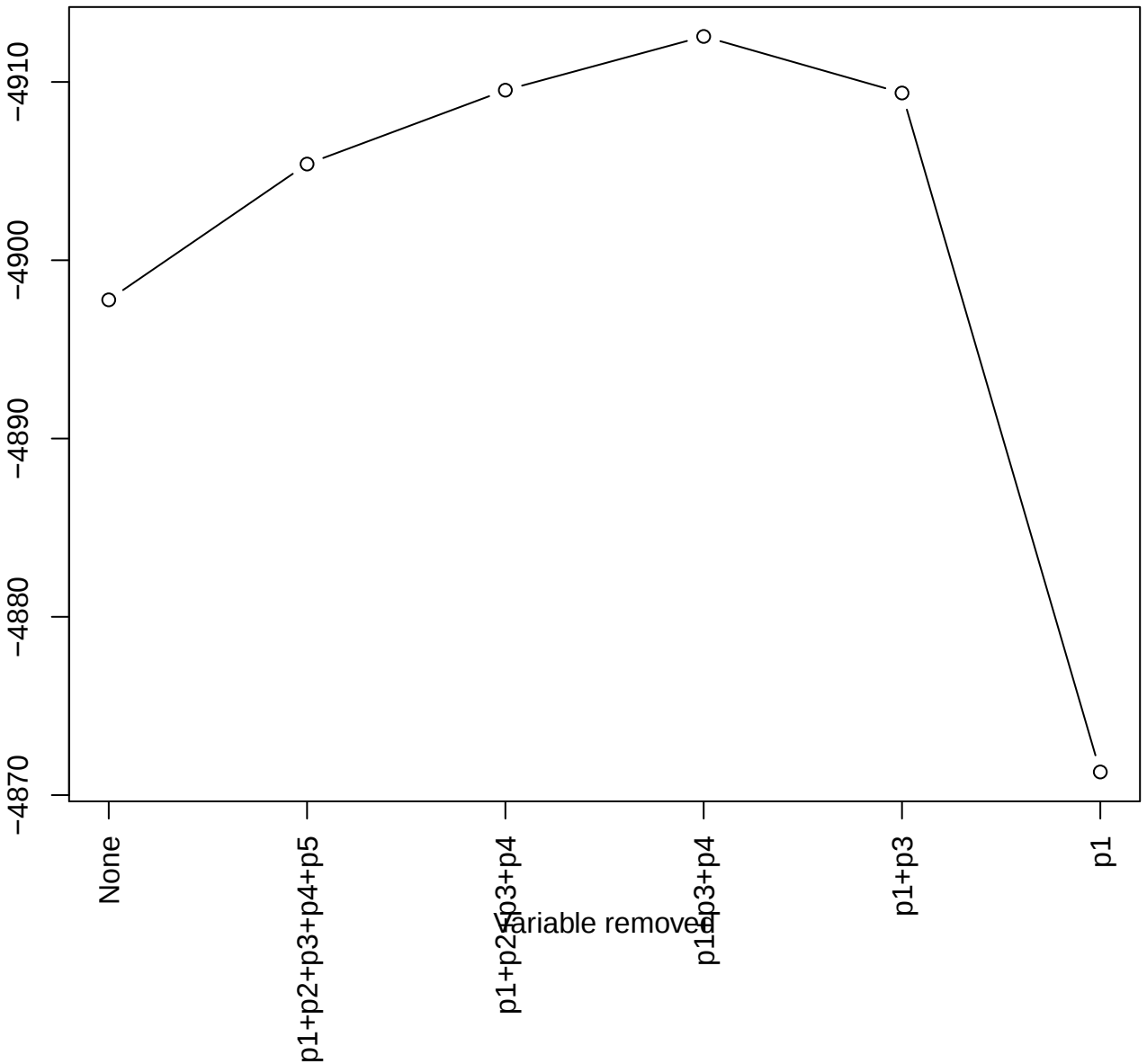
AIC v. variables (H)
