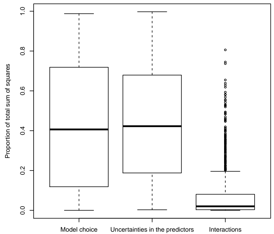
5% uncertainty in the predictors
