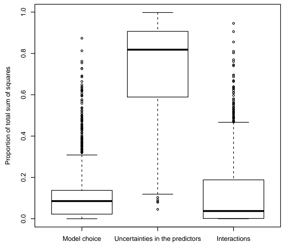
50% uncertainty in the predictors
