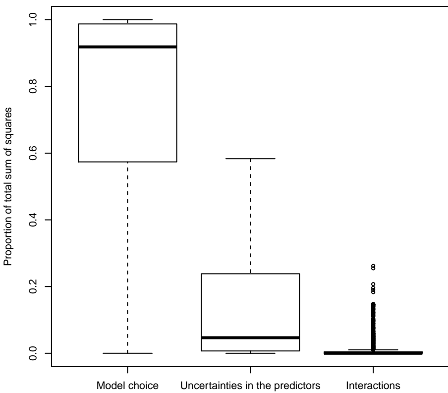
0% uncertainty in the predictors
