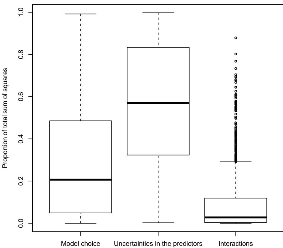
10% uncertainty in the predictors
