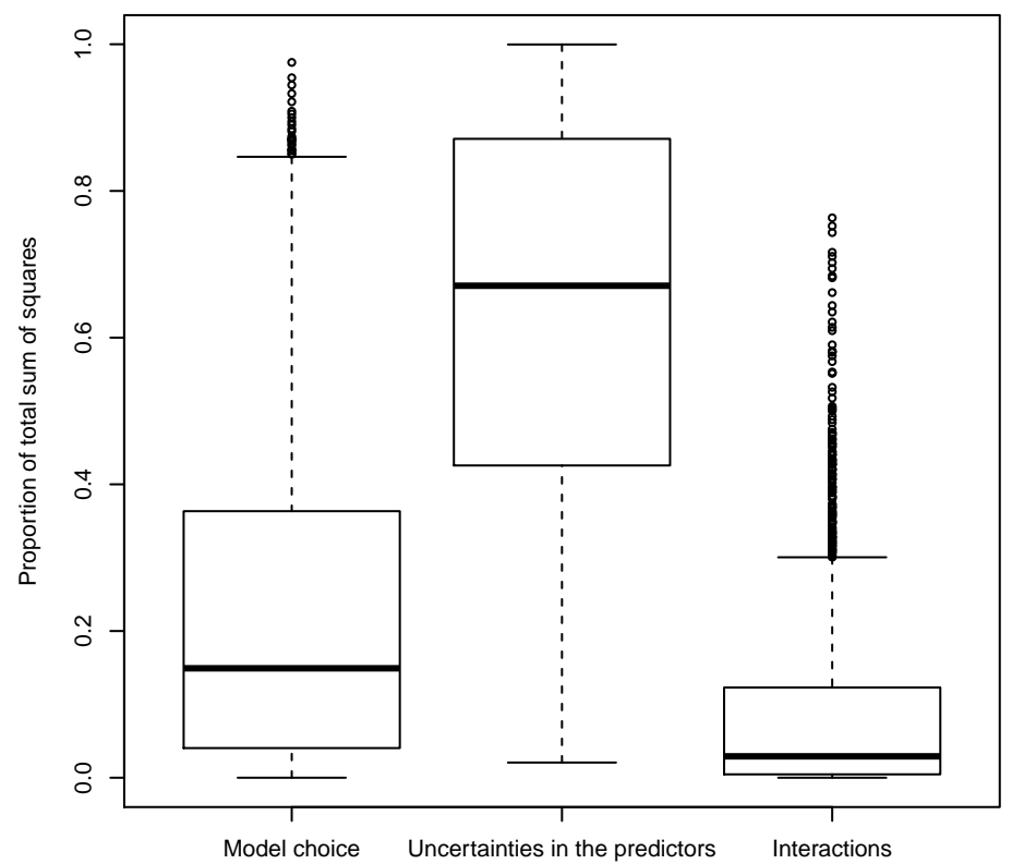
15% uncertainty in the predictors
