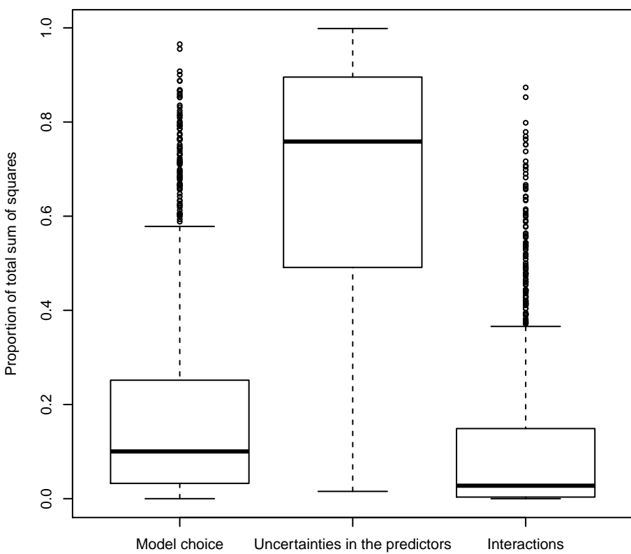
20% uncertainty in the predictors
