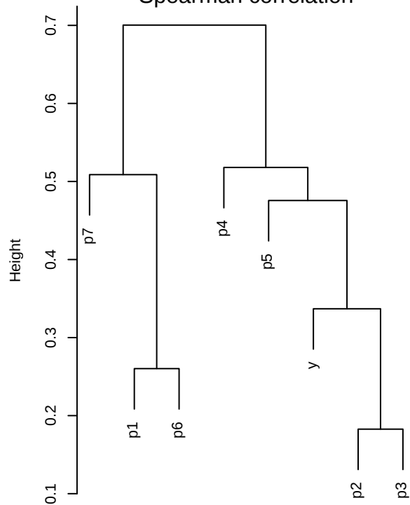
Dissimilarity = 1 - |Correlation| Spearman correlation
