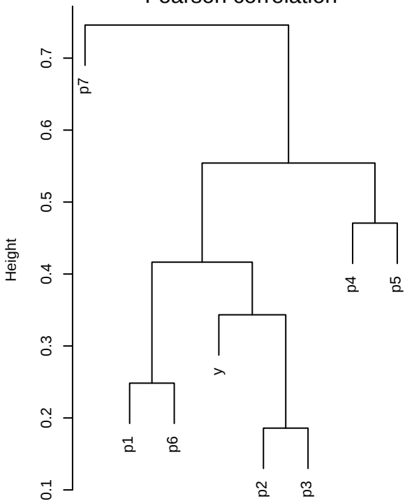
Dissimilarity = 1 - |Correlation| Pearson correlation
