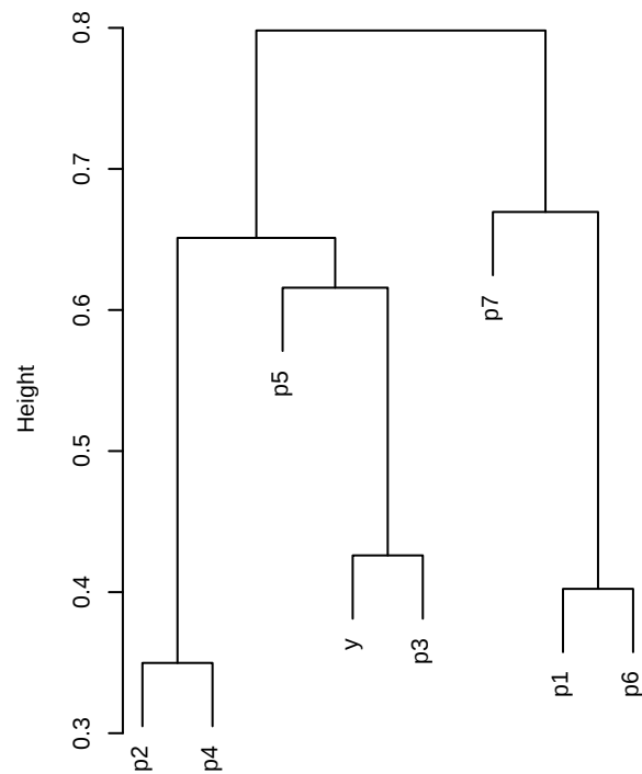
Dissimilarity = 1 - |Correlation| Kendall correlation
