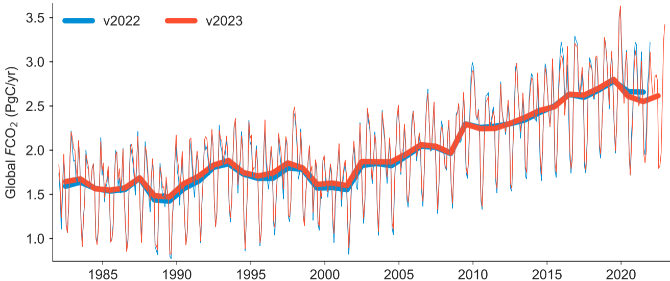
GCB-2023: OSETHZ-GRaCER v2023.GCB compared with v2022.GCB
